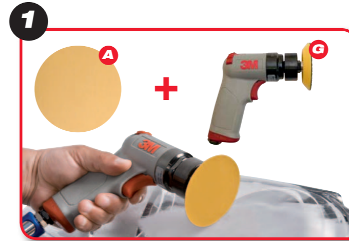
1 A - 3M™ Hookit™ Abrasive Disc 255P P500* G - 3M™ Random Orbital Pistol Grip Sander *P240 can be obtained for harder plastics
