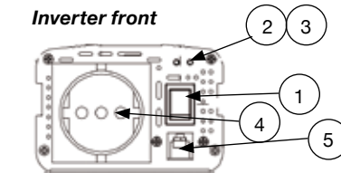
Inverter front
