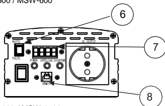
MSW-1000 / MSW-1500
