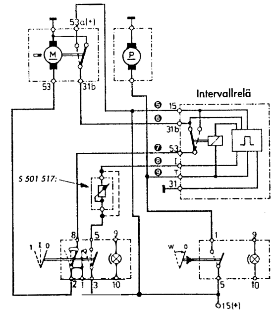
Inkopplingsexempel Connection example
